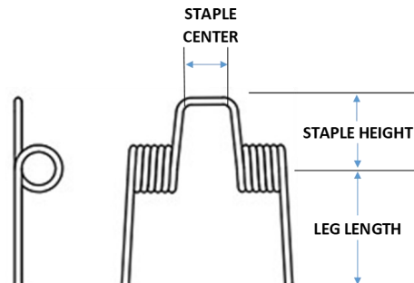
6 COILS/SIDE (12 TOTAL COILS) LEFT & RIGHT HAND WOUND
